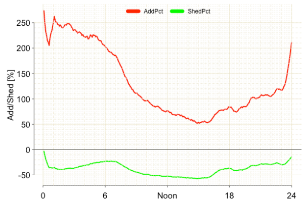
Figure 6 Thermal mass-enabled instantaneous feeder load adding/shedding, expressed as percentage, based on aggregated whole-building electric use
