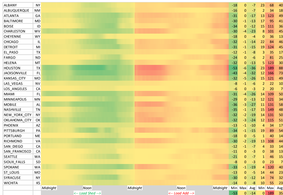
Figure 7 Heat map of thermal mass-enabled U.S. residential air-conditioning instantaneous percentage electric load-adding/load-shedding opportunities every 5 minutes. Note the increased add/shed opportunities because of increased air-conditioning loads in hot and humid southern climates, e.g., Houston, Texas, and Jacksonville, Florida
