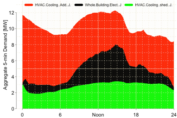
Figure 5 Thermal mass-enabled instantaneous feeder load adding/shedding based on aggregated whole-building electric use
