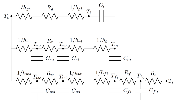
Figure 1 Building envelope model expressed as a thermal network (Corbin 2014)
