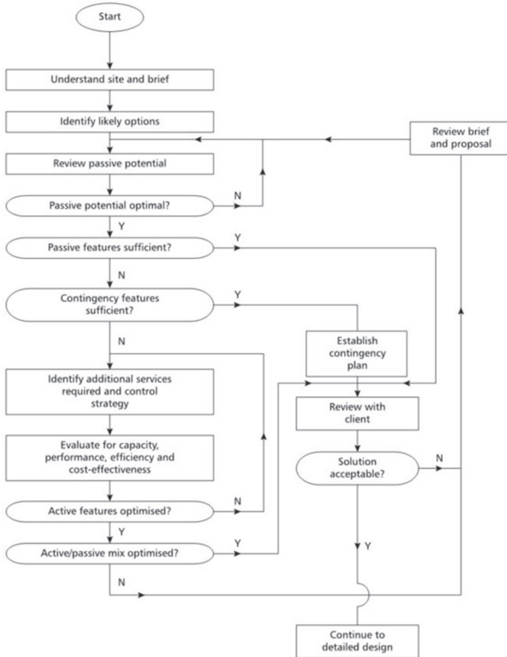
FIGURE WA5.6.1 CIBSE AM 10 flowchart for selecting a ventilation strategy.
