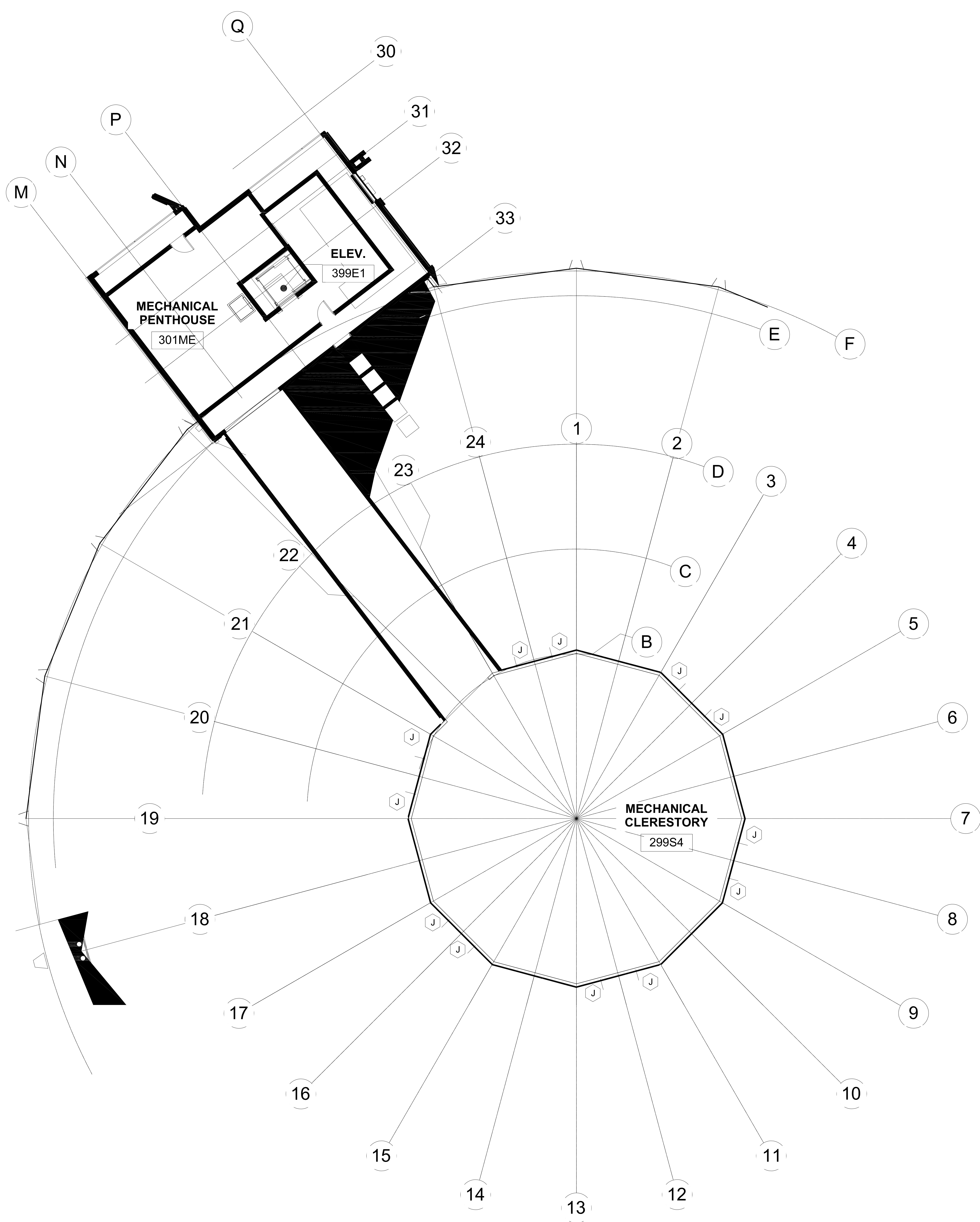
① MECHANICAL PENTHOUSE PLAN
