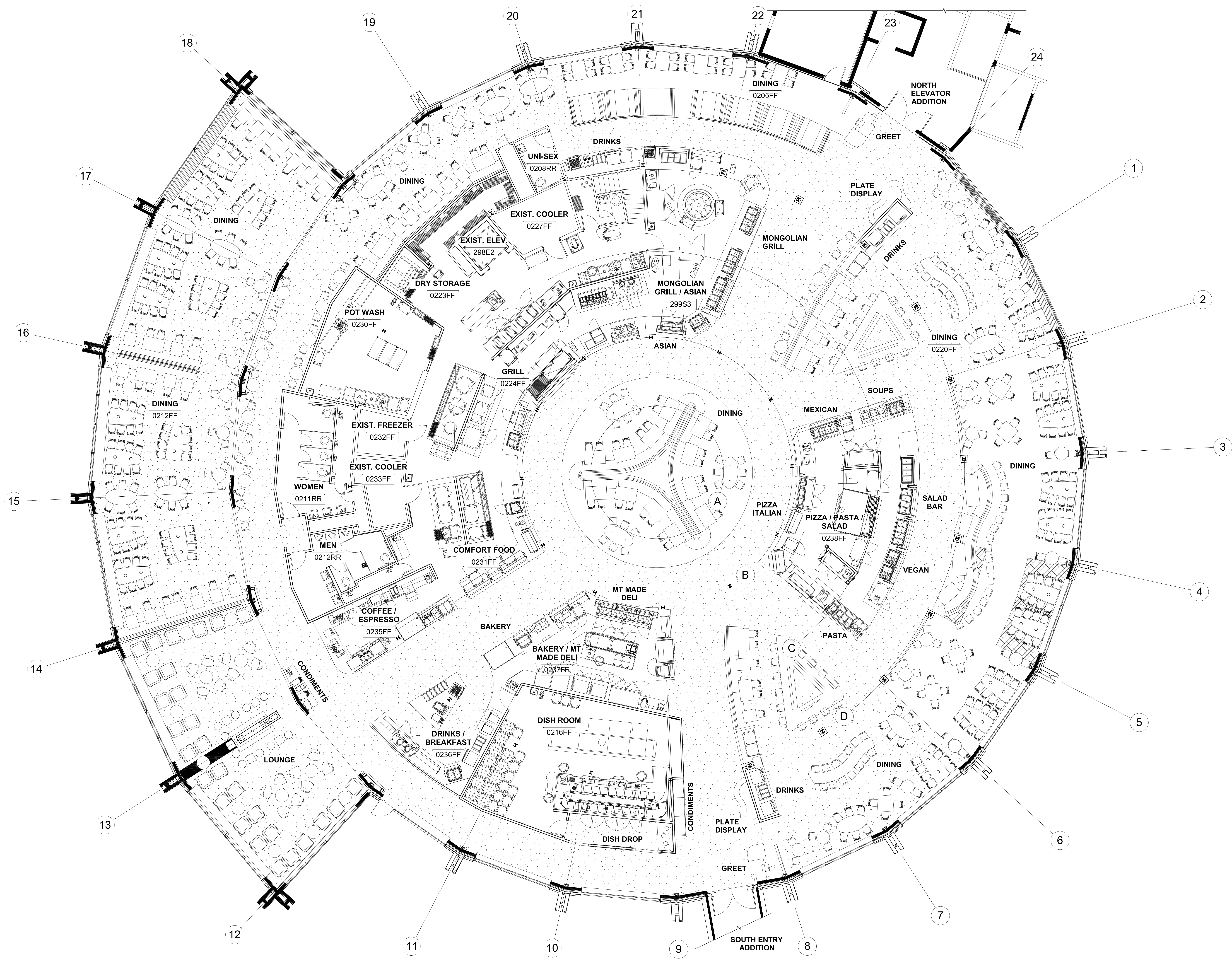
1 MAIN LEVEL REMODEL FLOOR PLAN
