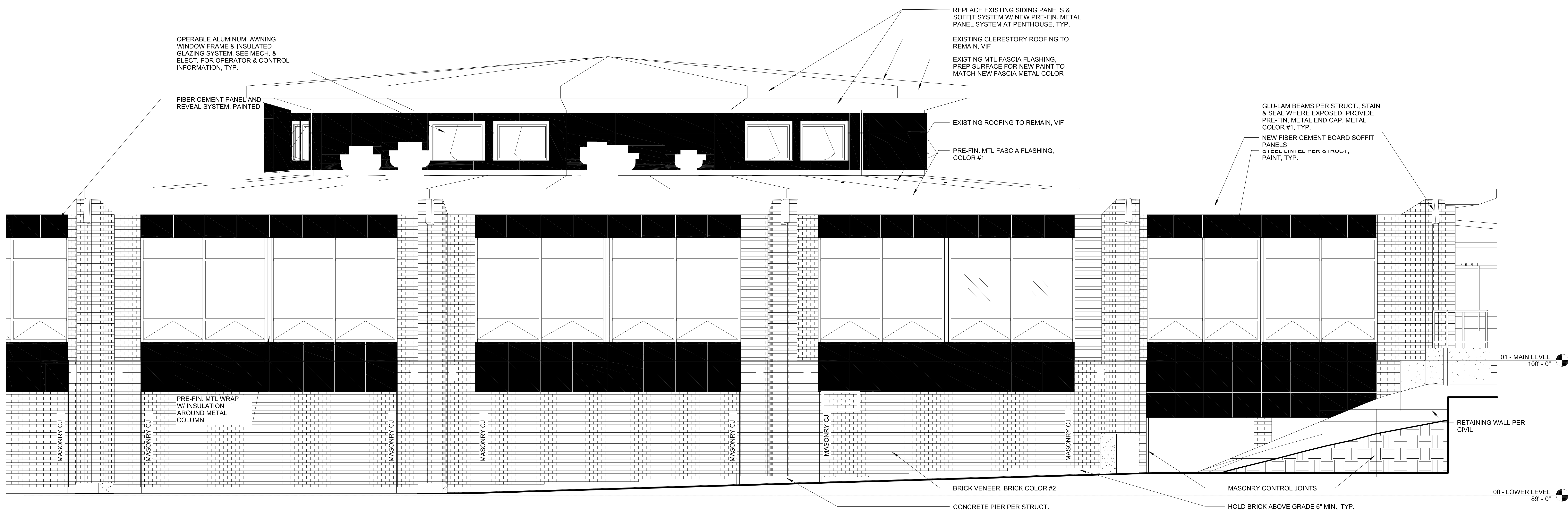
3 SOUTH ADDITION - SOUTH ELEVATION
