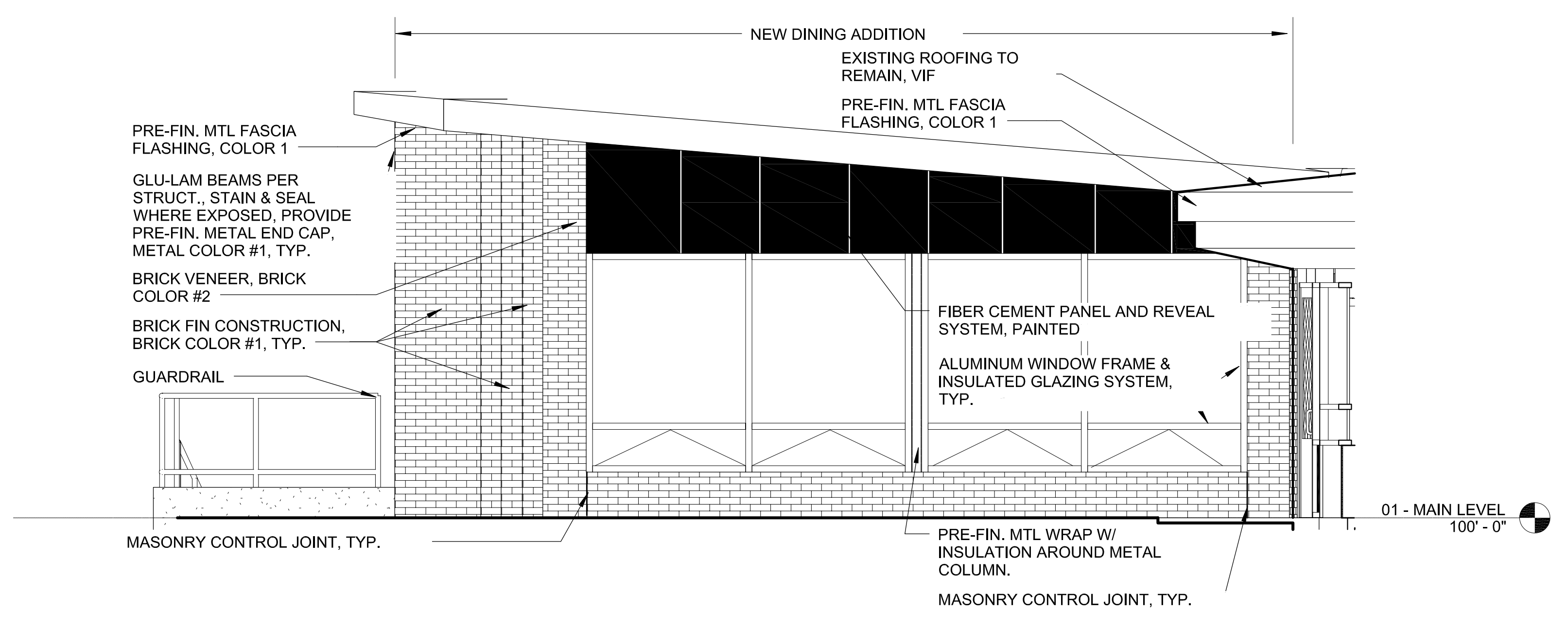
2 SOUTH ADDITION - EAST ELEVATION
