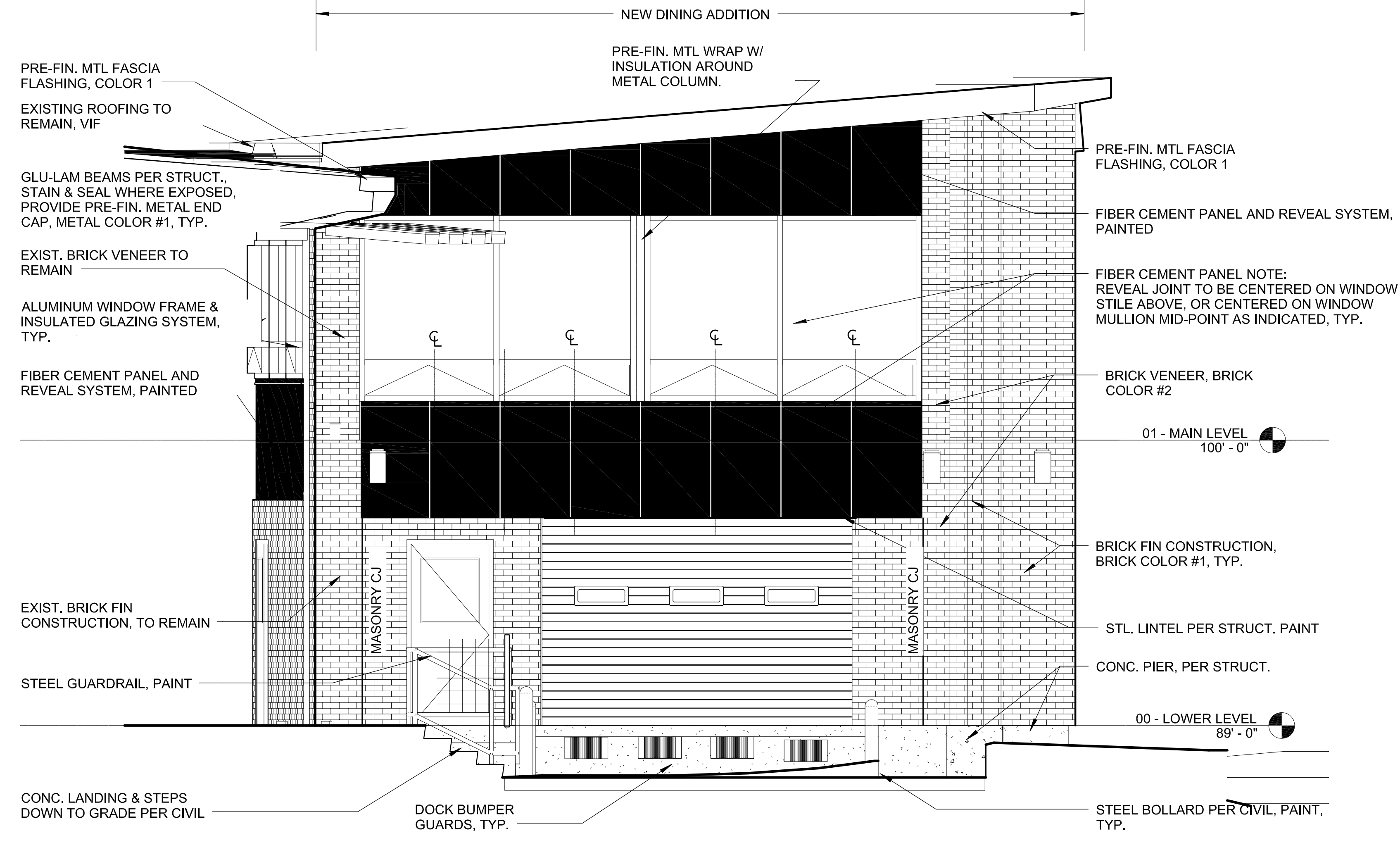
1 SOUTH ADDITION-WEST ELEVATION
