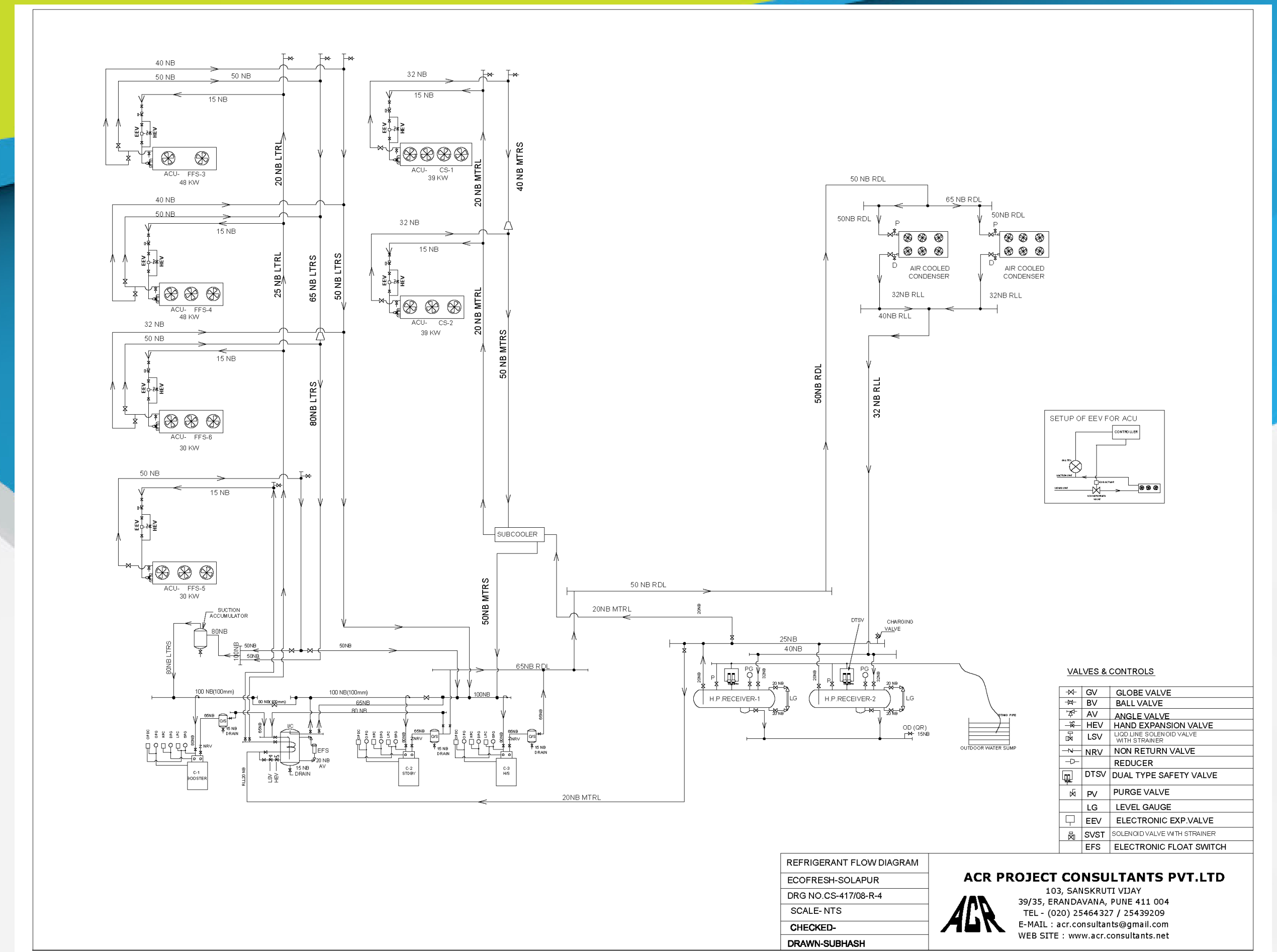
P&ID for Refrigeration System
