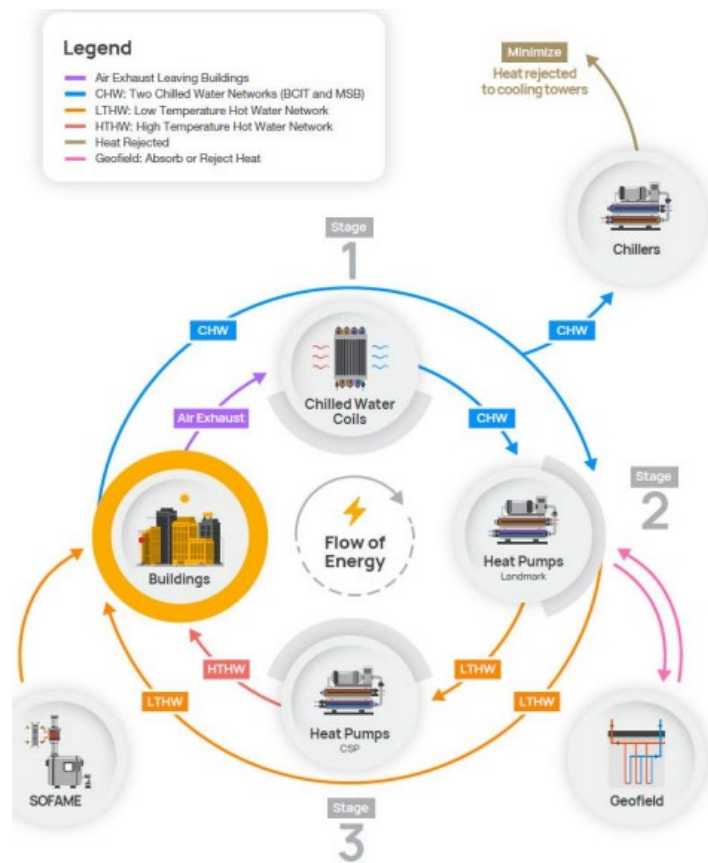
Online Figure 2. Cascading Heat Pump Approach. Source: Project LEAP, Decarbonizing St. George campus.
