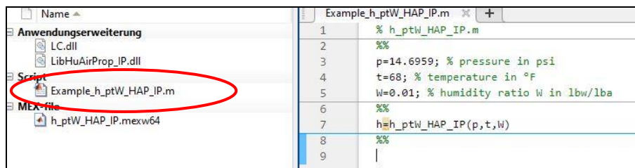
Figure 2.3.7: "Example_h_ptW_HAP_IP.m" M-file
