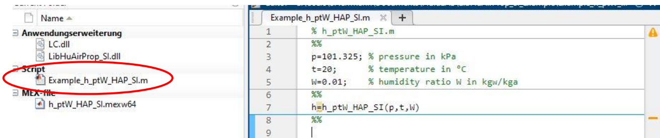
Figure 2.2.7: "Example_h_ptW_HAP_SI.m" M-file
