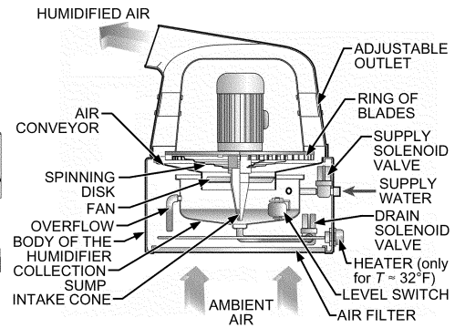
C. CENTRIFUGAL ATOMIZING STATION (Adapted from Lazzarin et al. 2004)
