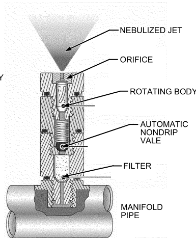
E. HIGH-PRESSURE SWIRL JET NOZZLE (Adapted from Lazzarin et al. 2004)
