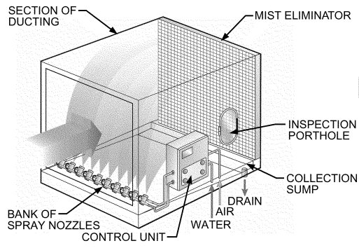
A. COMPRESSED-AIR NOZZLE HUMIDIFIER WITH MIST ELIMINATOR (Adapted from Lazzarin et al. 2004)
