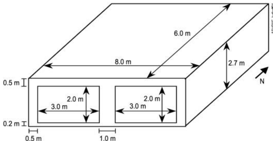
Figure 5-1 Isometric south windows—unshaded (Case 600).
