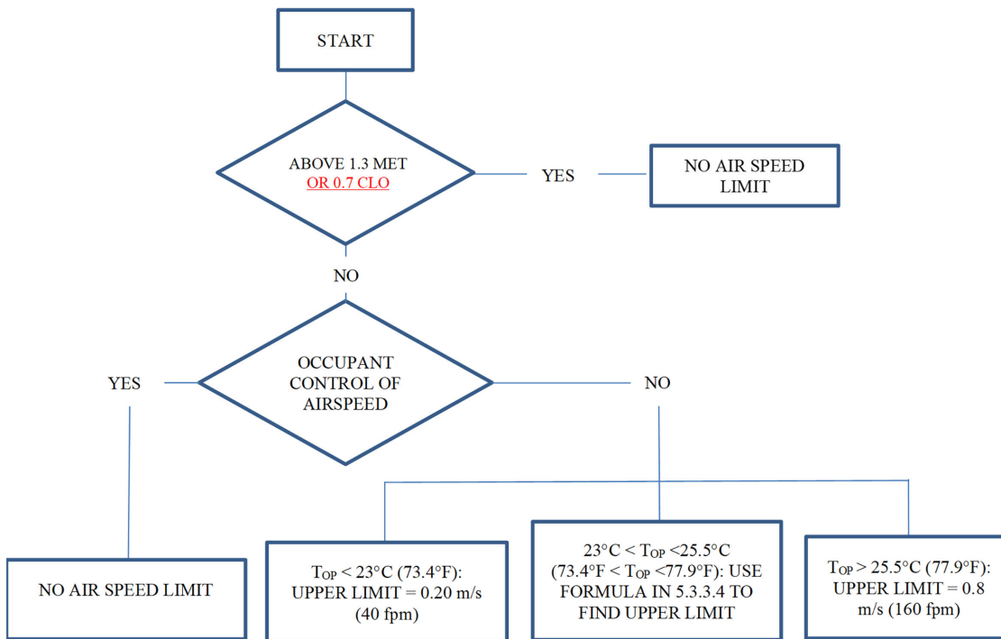
Figure 5.3.2C Flowchart for determining limits to air speed inputs in the Elevated Air Speed Comfort Zone Method.
