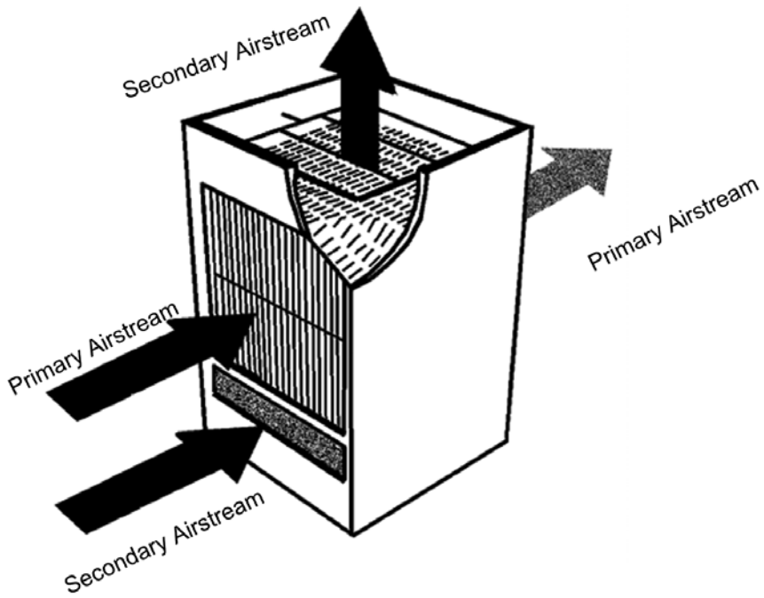
Figure 7 Indirect evaporative air coolers.
